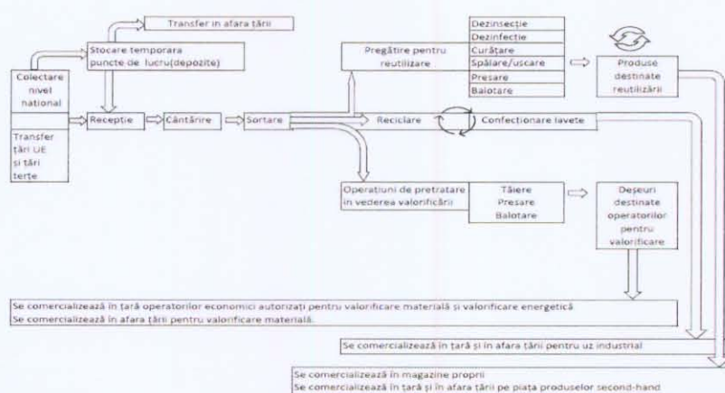
Schema flux
